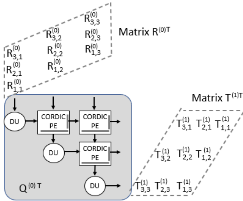
Fig. 4 Whole hardware for solving linear equations.
